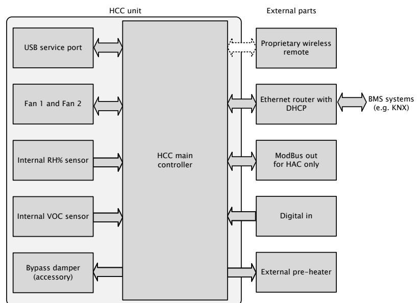
Overall system architecture schematics
