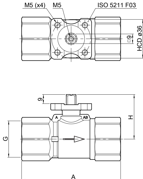
Fig. 7 2-way valves
